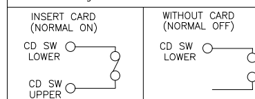
Circuit Diagram for Card Detect Switch
